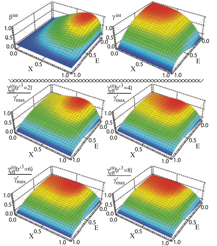
FIG. 6. (Color online) The top two graphs are the intrinsic hyperpolarizability and second hyperpolarizability as a function of X and E for a single-molecule system. The bottom four graphs show the intrinsic effective second hyperpolarizability of the aligned molecules with no energy corrections as a function of X and E for several r' values. The \beta contribution decreases as the distance of separation increases.
