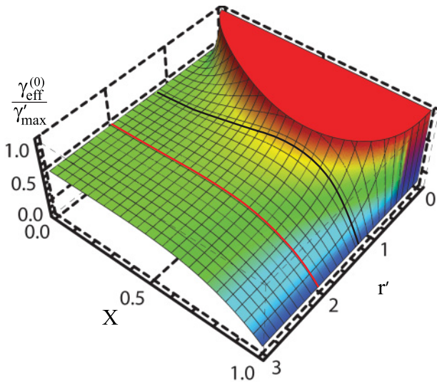
FIG. 7. (Color online) The semiclassical intrinsic effective second hyperpolarizability of two end-to-end molecules. The thick black line is the minimum separation distance given by the electromagnetic size of the molecule, or r' > \sqrt[3]{2} . The thick red line is the experimental limit of closest approach for spherical atoms which gives r' > 2 [23]. The red plateau is the region where \gamma_{\text{eff}}^{(0)}/\gamma'_{\text{max}} \leq 1 .
