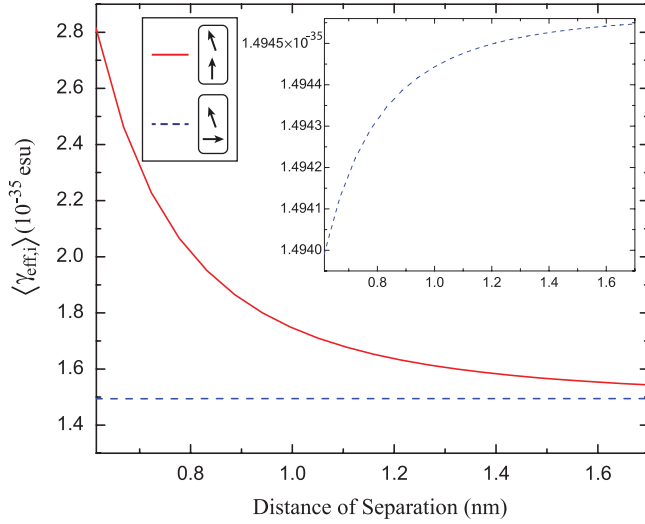
FIG. 9. (Color online) The contribution to the effective second hyperpolarizability of one freely rotating molecule that is coupled to a second molecule. The second molecule is held in both the direction perpendicular and the direction parallel to the applied field while the other is free to move. The temperature is 297 K and the poling field is 10^6 StatV/cm.
