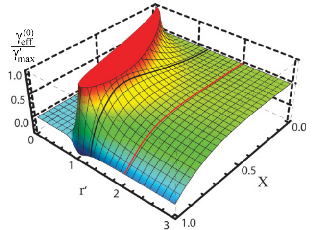
FIG. 5. (Color online) The intrinsic effective second hyperpolarizability of two interacting molecules. The thick black line is the lower limit of the center-of-mass displacement given by the condition r' > \sqrt[3]{2} . The thick red line is the experimental limit of closest approach for spherical atoms and molecules with large polarizabilities, r' > 2 [23]. The values that exceed the semiclassical limit have been removed from the diagram and are shown as the red plateau.
