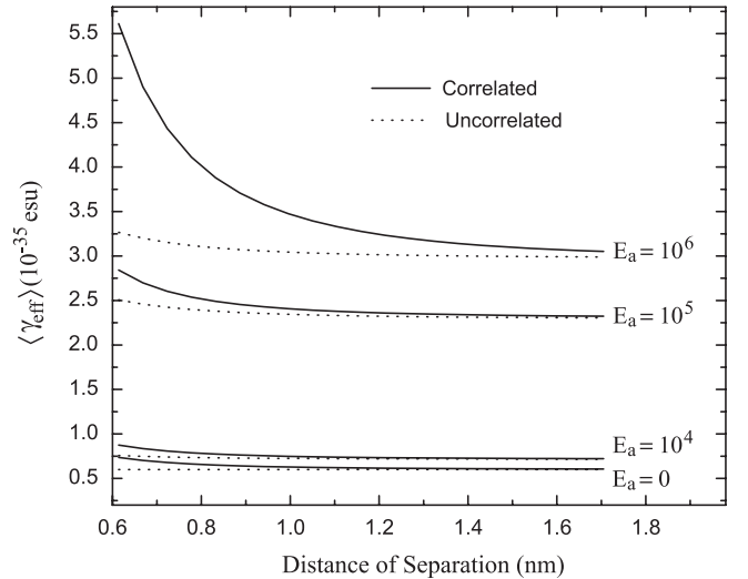
FIG. 8. The effective second hyperpolarizability of two interacting p NA molecules at a temperature of 297 K, where the separation vector between the two molecules is along the direction of the applied field. The molecules are freely rotating, where the alignment is a result of the applied electric field in units of StatV/cm. The solid curves include interactions between polarized molecules and the dotted curves include only the effects of the applied electric field.
