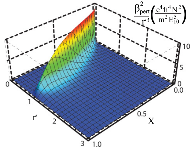
FIG. 4. (Color online) The cascading contribution of \beta_{\text{pert}}^2/r'^3 . The perturbed Hamiltonian keeps the function from diverging as r' \rightarrow 0 .
